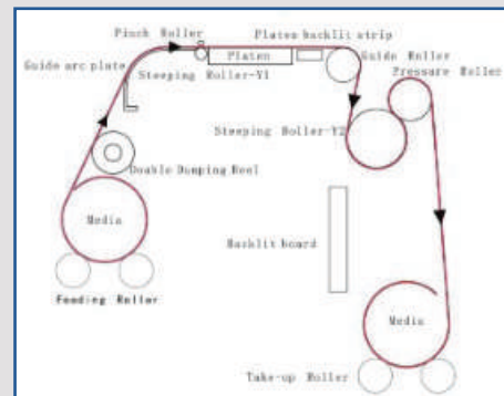
DOUBLE ROLLER FEEDING
