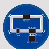
White Ink Recirculation System
